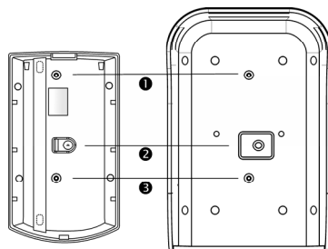
Figure 2 Attaching the detector to the Hood
