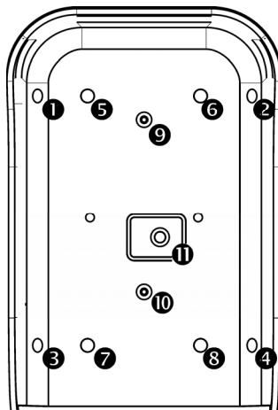
Figure 1: MH-5 Mounting holes
