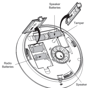
Figure 3-2: Inserting the batteries
