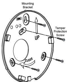
Figure 4-1: Attaching the mounting bracket
