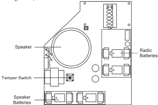
Figure 3-3: Inserting the batteries #2
