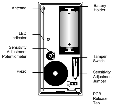
Figure 1: EL-2607 (Cover Off)
