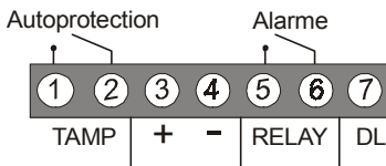
Figure 1: Bornier
